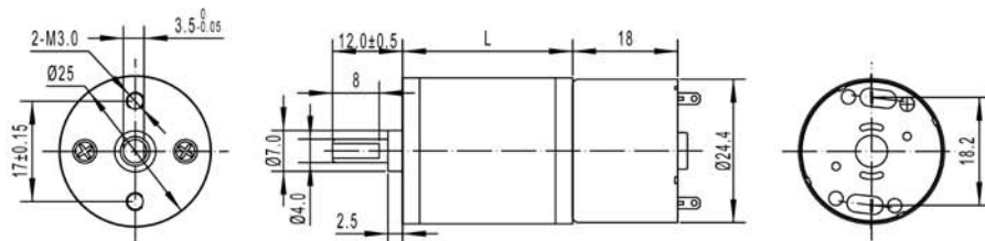
Gear Motor Dimensions (mm)
