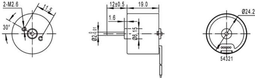
Motor Dimensions (mm)
