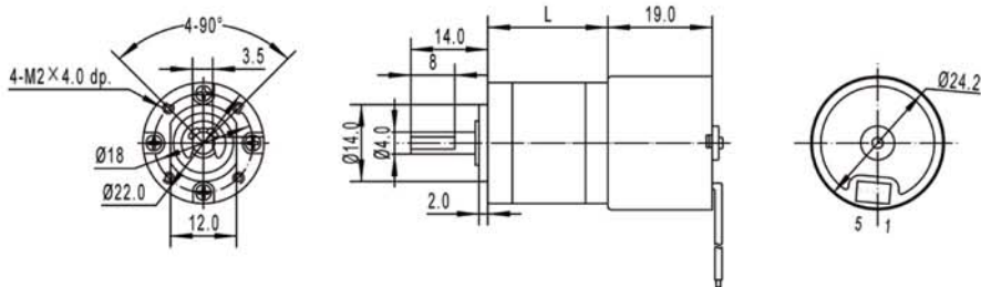
Gear Motor Dimensions (mm)
