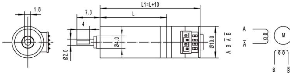
Gear Motor Dimensions (mm)
