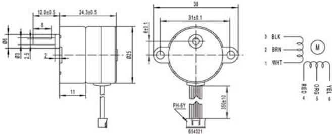
Gear Motor Dimensions (mm)
