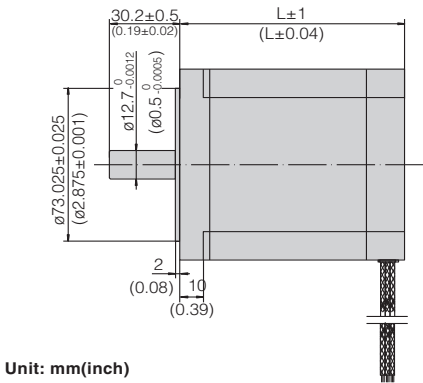
Unit: mm(inch)
