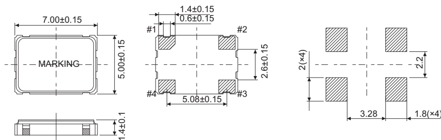
Example of a Terminal Land Pattern
