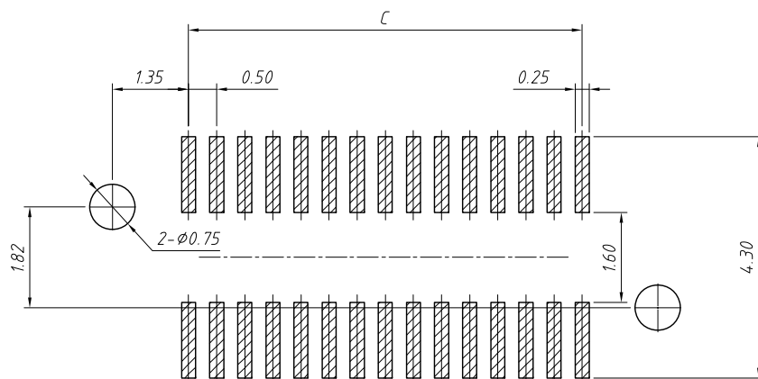
PCB LAYOUT
